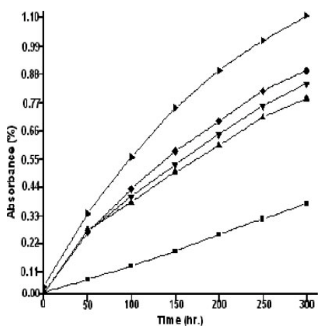
Figure 7 Rate of hydroxyl group formation in E copolymers during photodegradation (100, 200, and 300 h) by 2/MAO catalyst system: (■) E, (▲) E-H, (▼) E-U, (◆) E-MMA, (►) E-AA.
